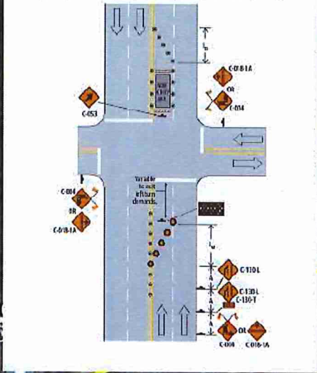
Figure 11.7: Left Lane Closure For 11th - Roll-In Intersection - Short and Long Duration
