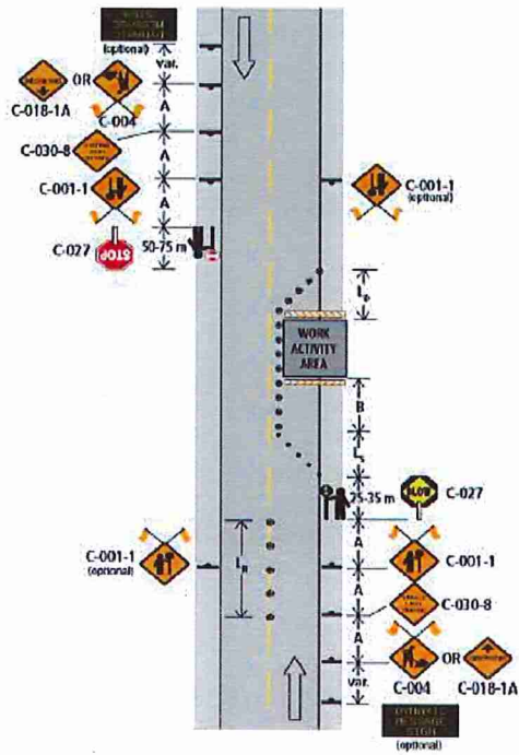
Figure 7.8: Lane Closure with TCPs – Single Lane Alternating – Short and Long Duration
